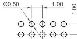
Recommended PCB Layout General TOL: ±0.05
