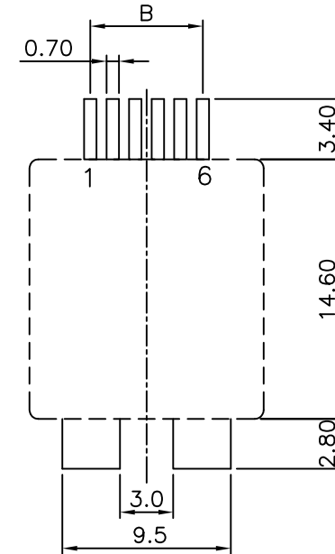
RECOMMENDED PCB LAYOUT AS VIEWED FROM COMPONENT SIDE
